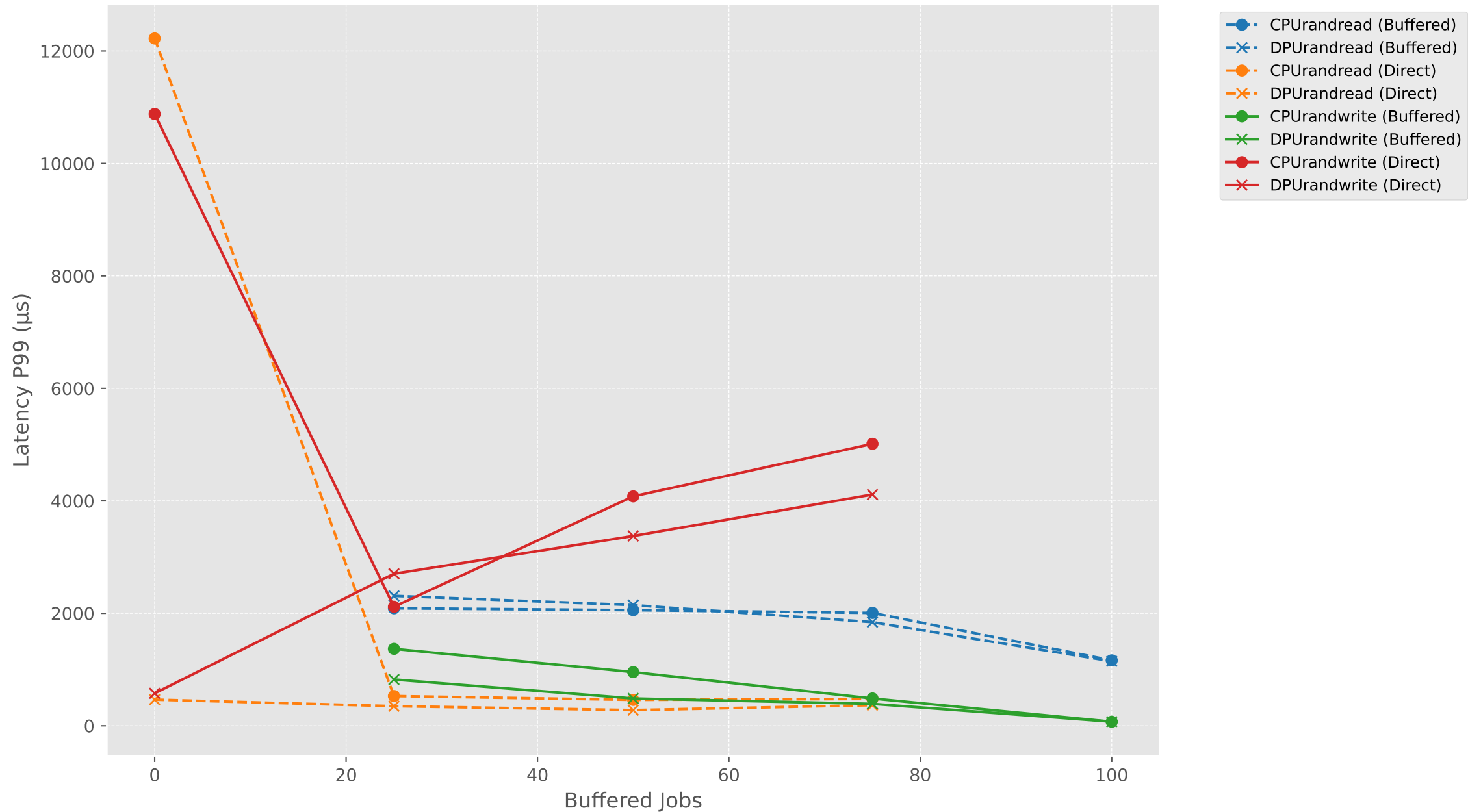
Latency P99 vs Buffered Jobs (mixed) - RAND (CPU vs DPU)
